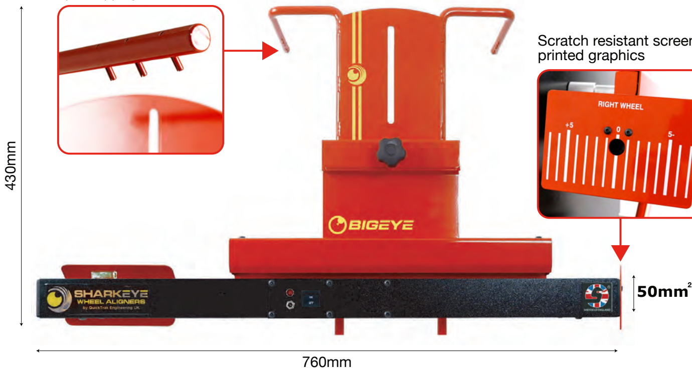
Tyre Gripping Pins
